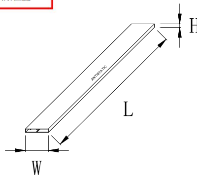
Fig.1- Tube pack for TO-247-4
